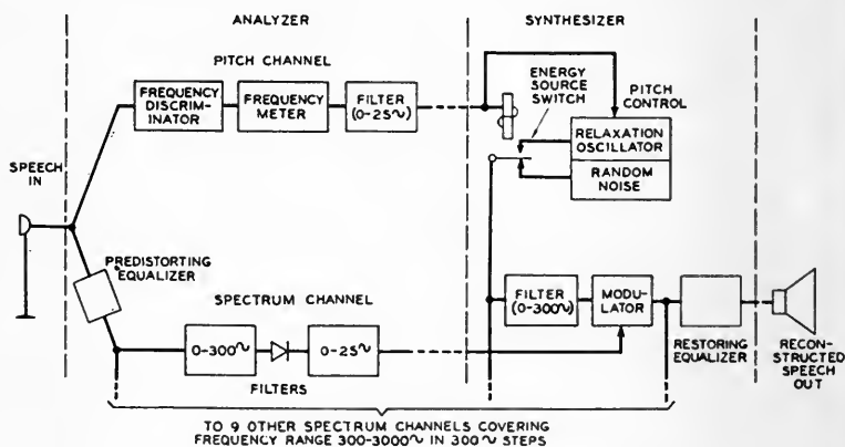
FIG. 2. Schematic arrangement of the Vocoder.
